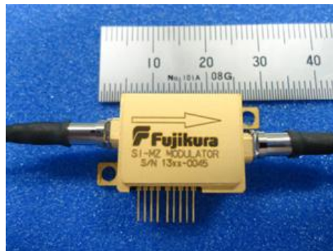
Evaluation module of 10 Gbps silicon optical modulator
