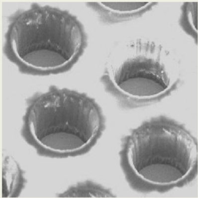
KrF excimer laser-drilled micro-vias
