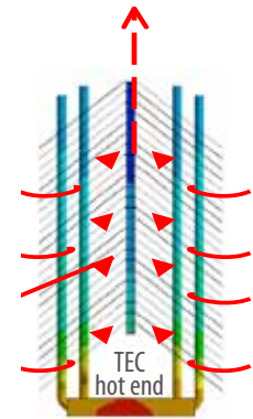
Figure 3: The tubes transfer heat from the hot end of the TEC, which create a temperature difference around the aluminum foil surfaces. This heats up the air near the surface of the foils, which rises, and drags in cooler air from the surrounding
